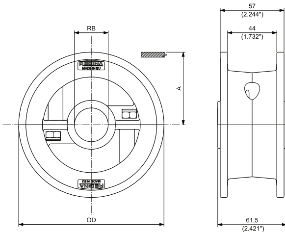
ROUNDBORE- IDLER
